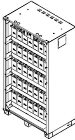
BRUA463284 Isometric View
